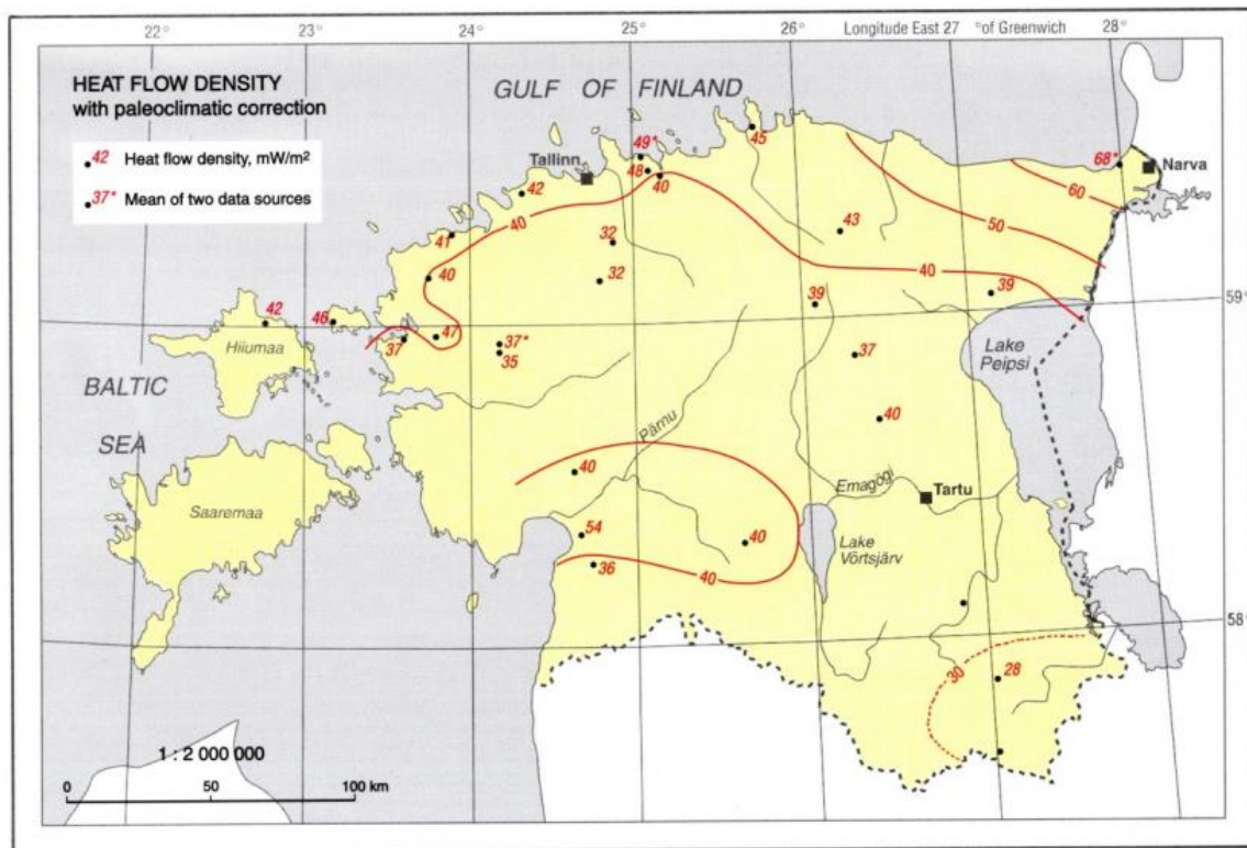
Exhibit 9: Improved heat flux density map with respect to past climate change effects that better describes the heat flow coming from deeper underground (Jöeleht, 2002).
