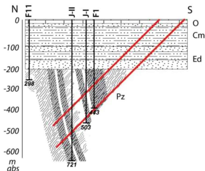
Exhibit 15: Geologic Interpretation from the Jõhvi drill holes. The dark colours represent gneisses while the light colours represent granitic rocks (primarily quartzite).
