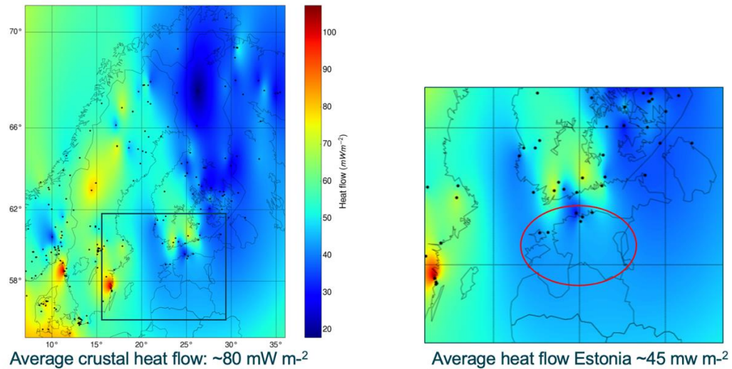
Exhibit 8: Conservative view of measured heat flux density (Jõeleht, 2002). The figure shows only reliable data for which temperature data have been available, and it has been possible to check the absence of effects related to water flow. When excluding the Northeast Estonia, the rest of the Estonia has a heat flux density in the range of 30-40 mW / m².
