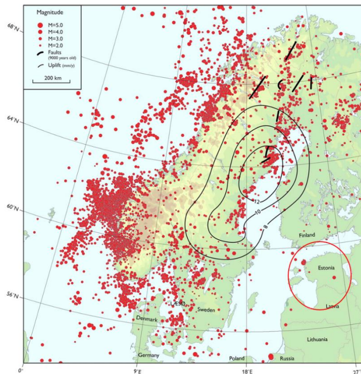
Exhibit 6: Map of seismicity in Scandinavia from January 1970 to December 2004. Contour lines show post-glacial uplift in millimetres per year. 21
