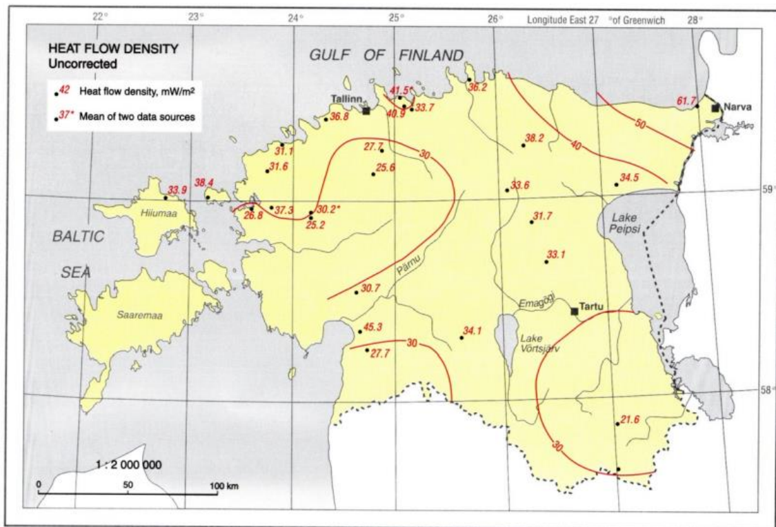
Exhibit 8: Conservative view of measured heat flux density (Jõeleht, 2002). The figure shows only reliable data for which temperature data have been available, and it has been possible to check the absence of effects related to water flow. When excluding the Northeast Estonia, the rest of the Estonia has a heat flux density in the range of 30-40 mW / m².
