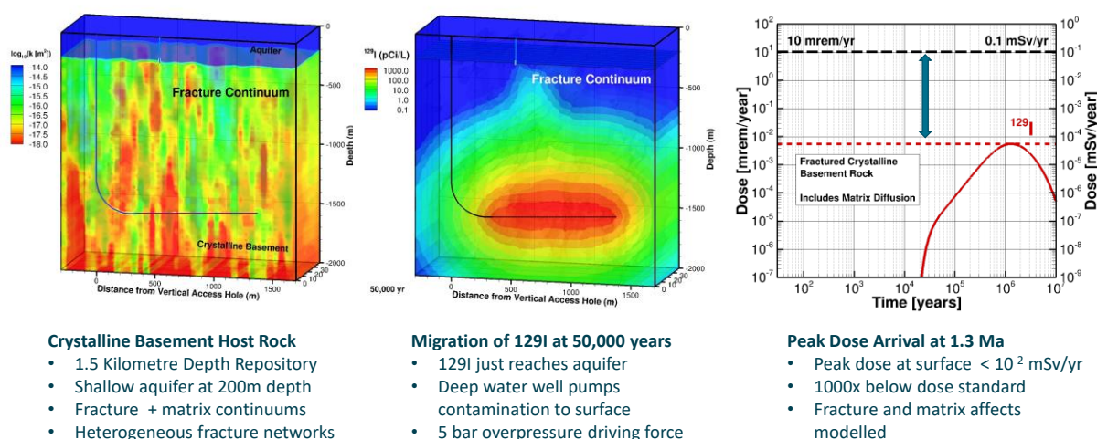
Exhibit 17: Preliminary generic safety calculations for a horizontal repository in crystalline basement at a depth of 1.5 km 39
