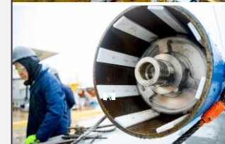
Initial full-scale PWR canister test on 23 February 2023
